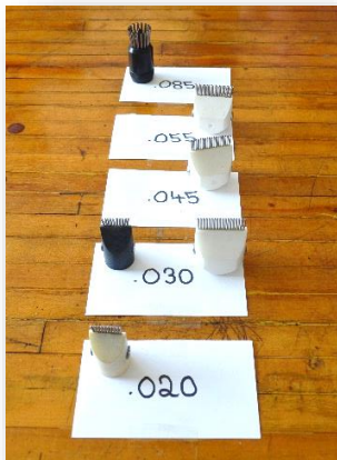
Left to right: Explanation of the various nozzle apertures designed to control droplet size and placement. Support vehicle with self-contained herbicide concentrate and diluent tanks and landing/loading platform.
